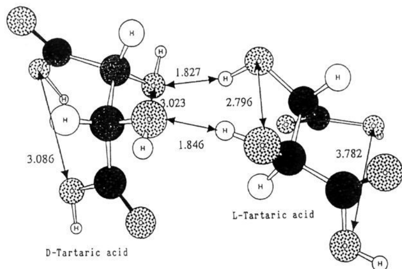
Figure 2. Diagram of the D-L two-hydrogen-bonding tartaric acid complex, showing selected distances between the atoms, as discussed in the text.
