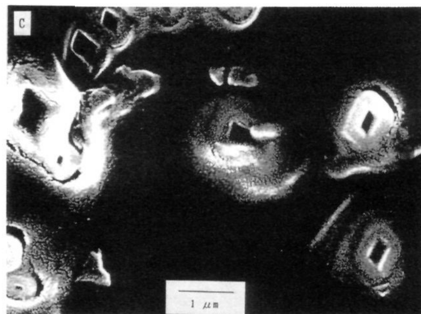
Figure 1. (A) Electron microscopic view (1000×) of the products of the reaction of TEOS dissolved in absolute ethanol containing DL-tartaric acid with ammonium hydroxide solution. (B) Close-up of the hollow tubes collected upon washing the reaction products. (C) Cross section of the tubes, showing the square inner shape and the outer diameter of 0.8–1.0 μm.
